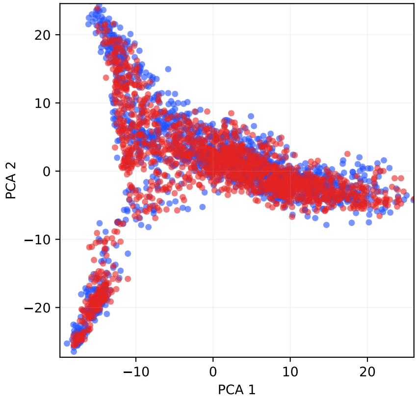
HaluEval (Layer 7)
