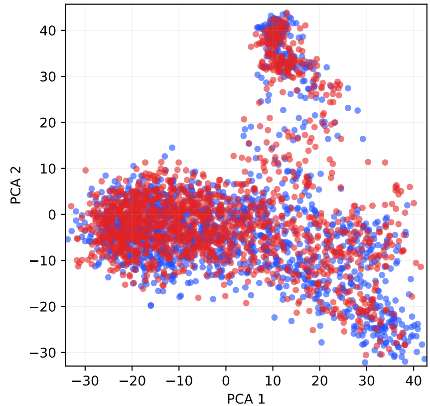
HaluEval (Layer 8)
