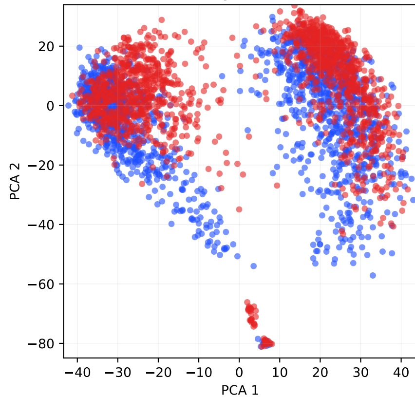
Belief Bank Constraints (Layer 24)
