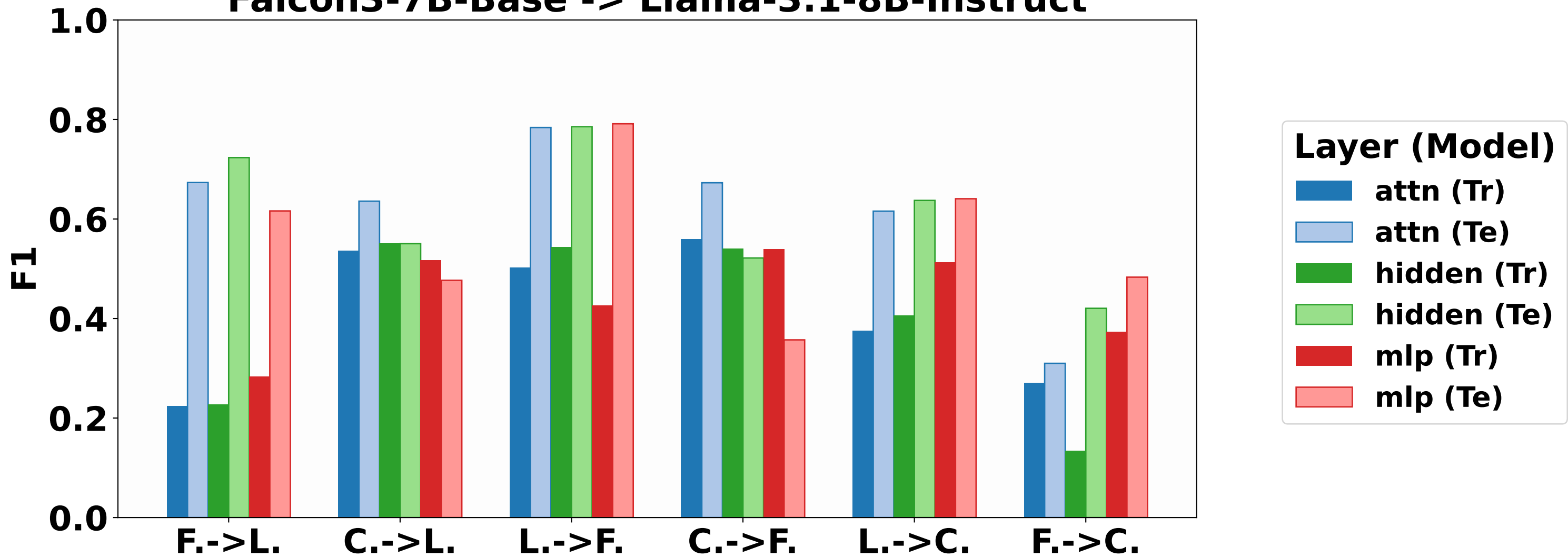
Falcon3-7B-Base -> Llama-3.1-8B-Instruct
