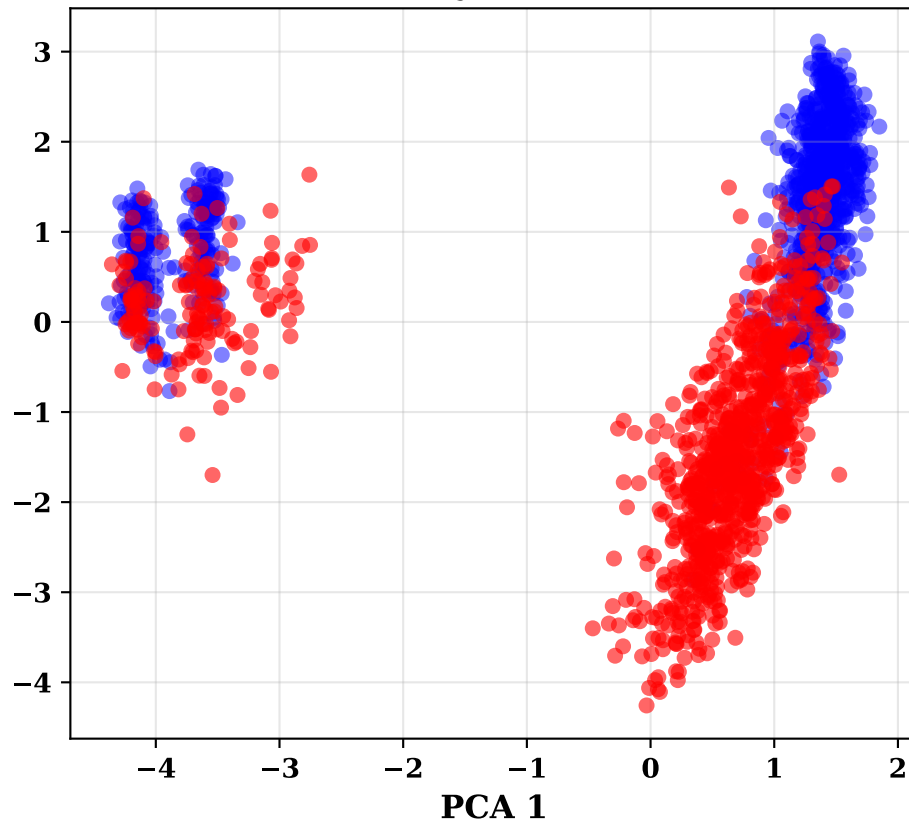
Belief Bank Facts (Layer 14)
