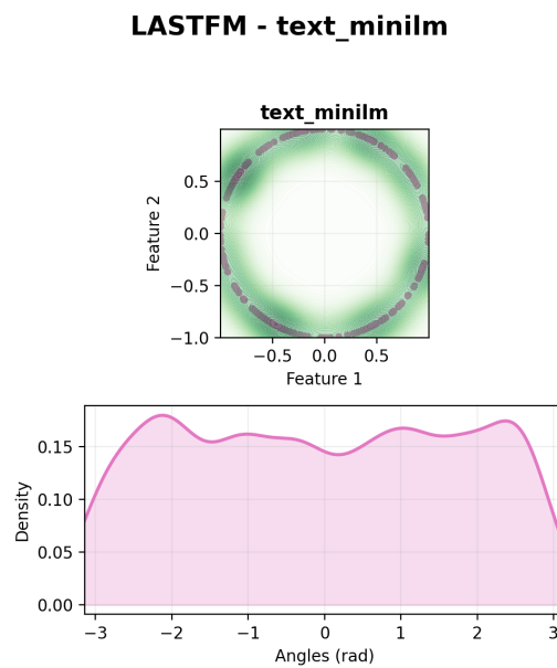
Figure 14: LastFM - Text embeddings (MiniLM)
