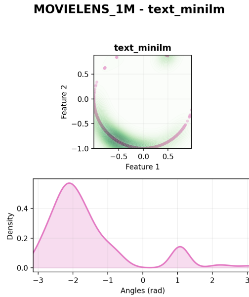
Figure 6: MovieLens 1M - Text embeddings (MiniLM)
