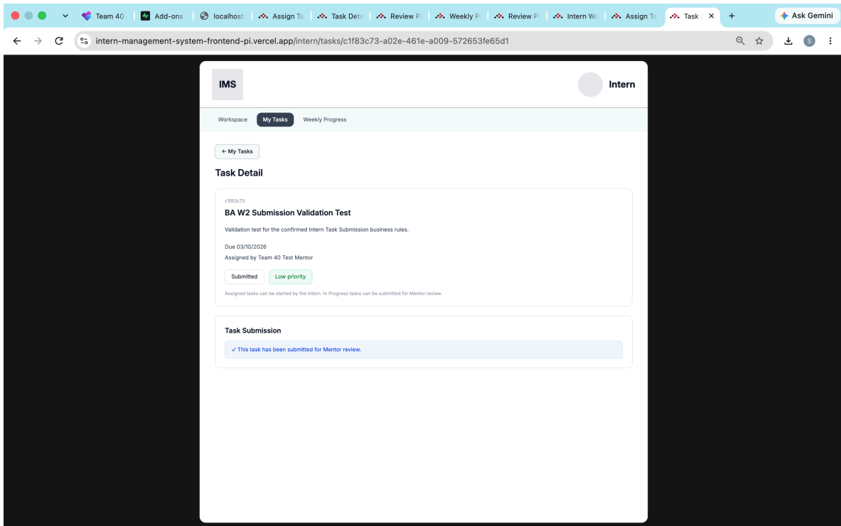
Figure 28. Defect evidence: attachment-only submission is accepted and moves to Submitted.
