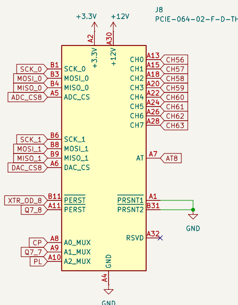
PCle x4: Unit 8
