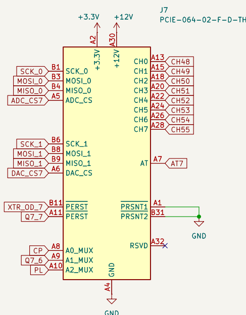
PCle x4: Unit 7
