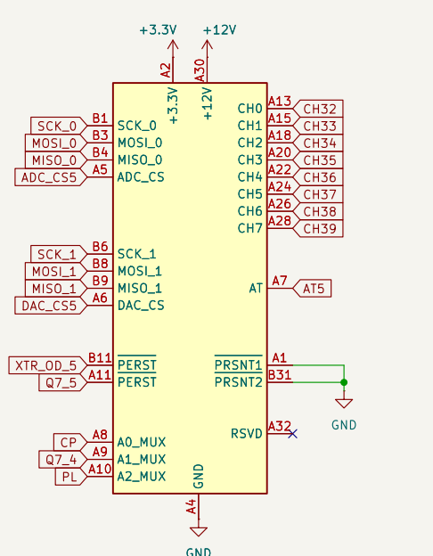
PCle x4: Unit 5
