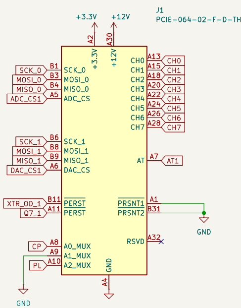
PCle x4: Unit 1
