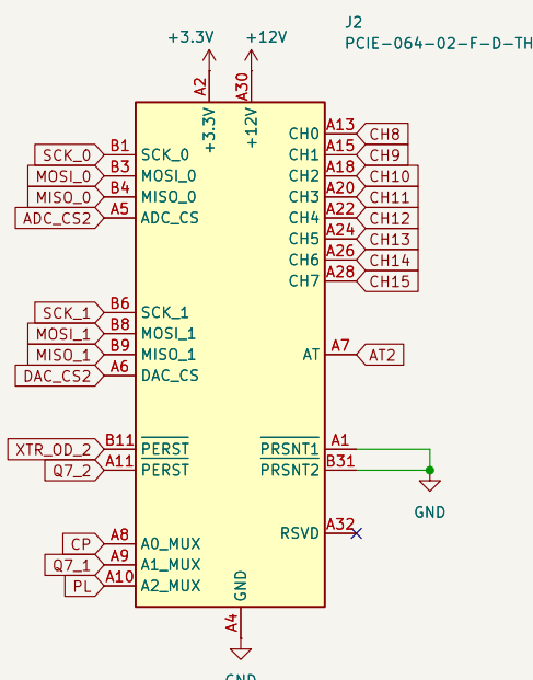
PCle x4: Unit 2
