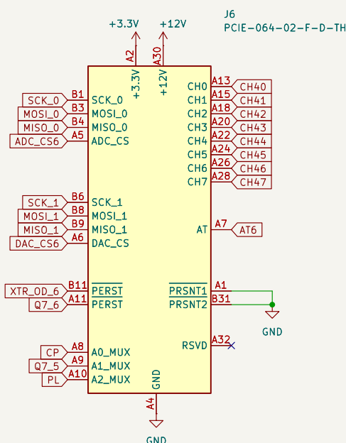
PCle x4: Unit 6
