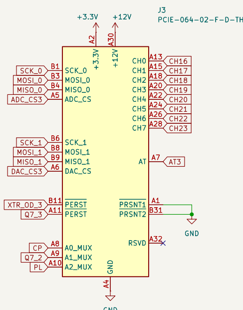
PCle x4: Unit 3
