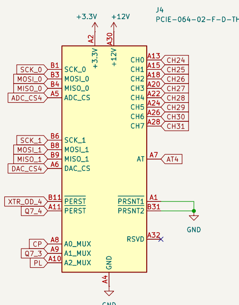
PCle x4: Unit 4
