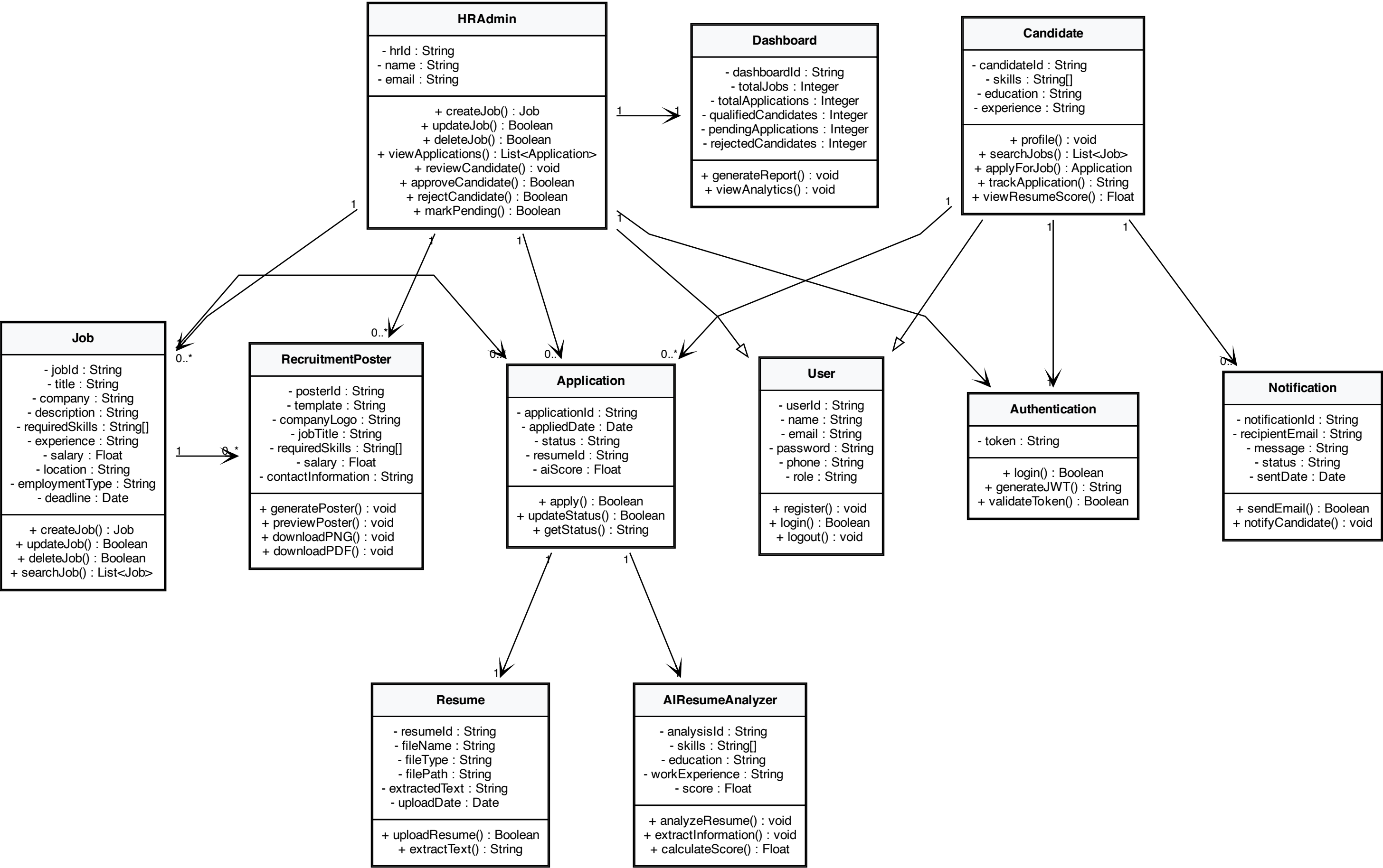
UML Class Diagram - AI-Powered Applicant Tracking System (ATS)
