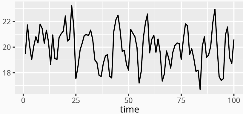
MA(1)
