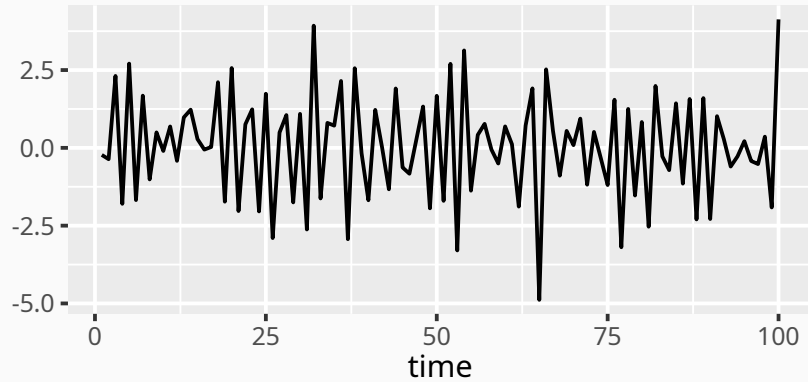
MA(2)
