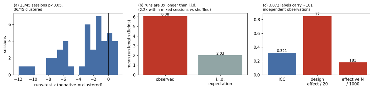
Figure 3. (a) runs-test z per session; (b) observed versus i.i.d. run length, pooled over all sessions; (c) ICC, design effect and effective sample size.
