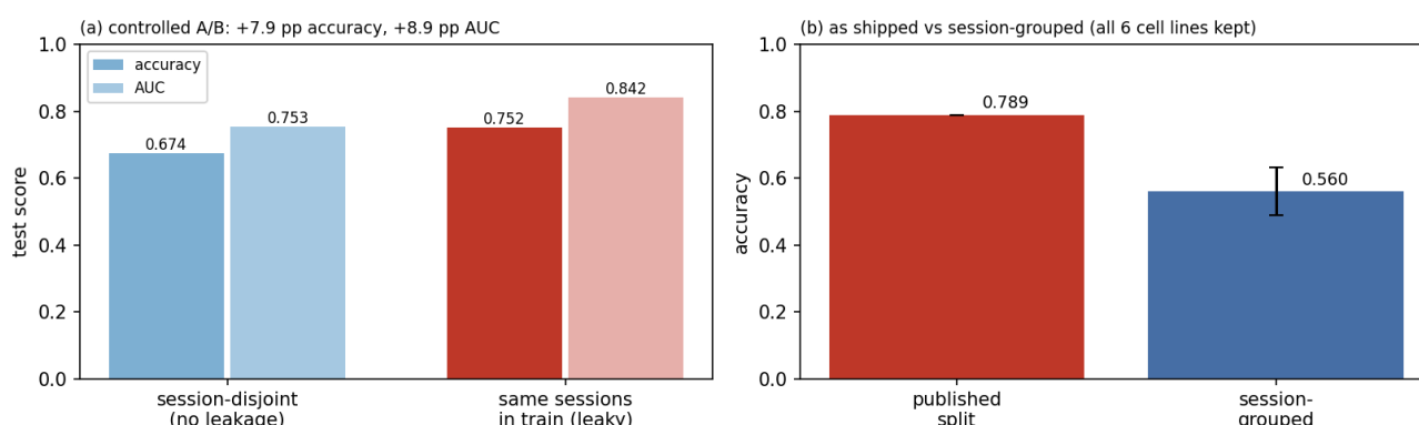
Figure 2. (a) controlled A/B (8 seeds; paired inflation +7.9 pp accuracy, +8.9 pp AUC; the gain is positive in every seed, 4.2–17.8 pp); (b) the shipped split versus a session-grouped split.
