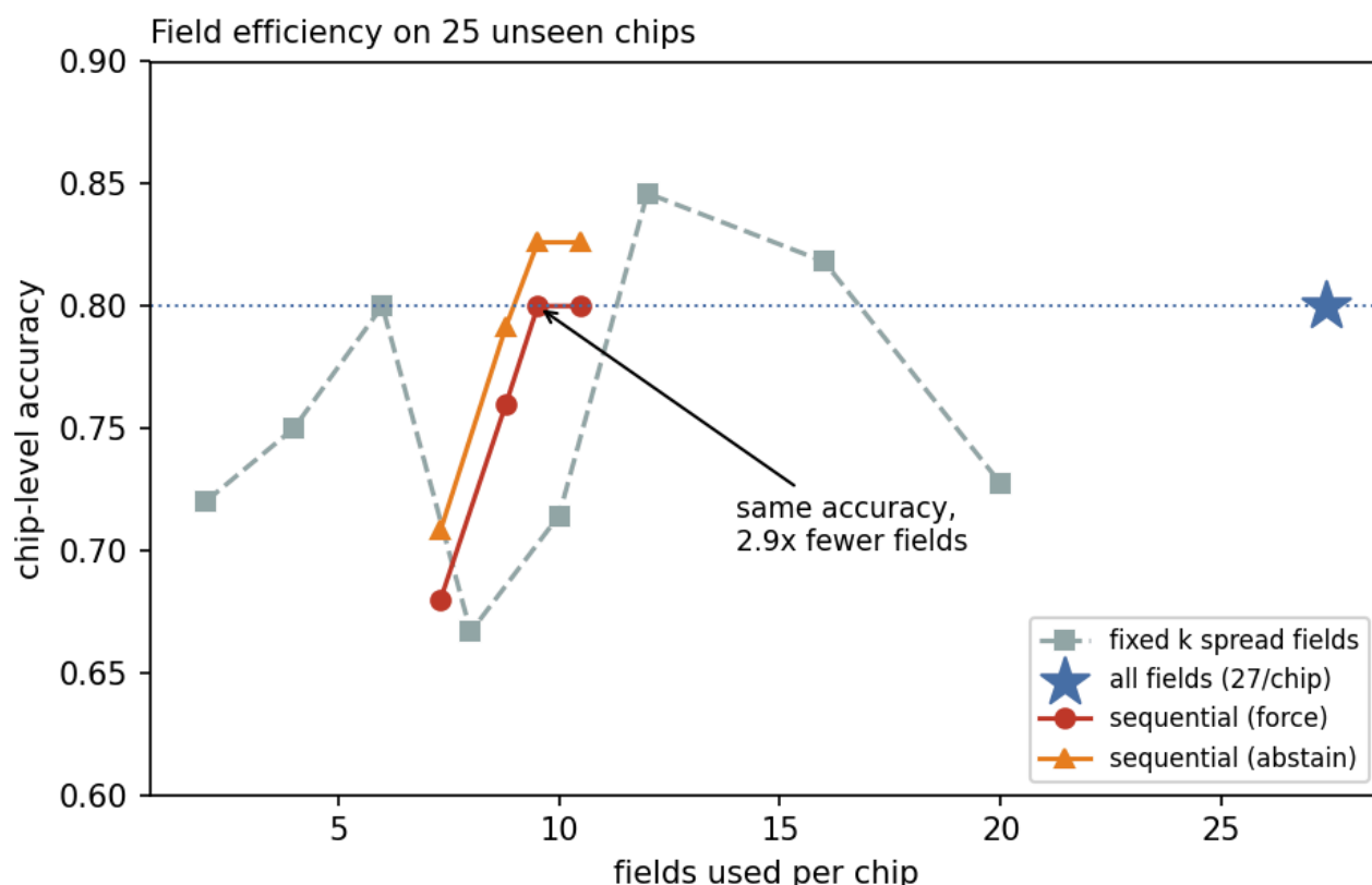
Figure 7. Accuracy against the number of fields used per chip.
