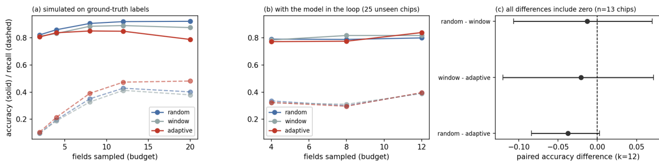
Figure 4. Policy comparison. (a) simulated on ground-truth labels; (b) with the model in the loop; (c) paired bootstrap differences at k=12 — all intervals include zero, so no ranking is claimed.
