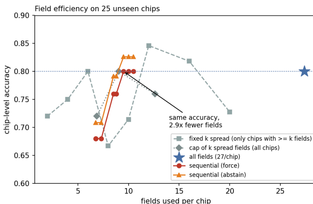
Figure 6. Accuracy against the number of fields used per chip.
