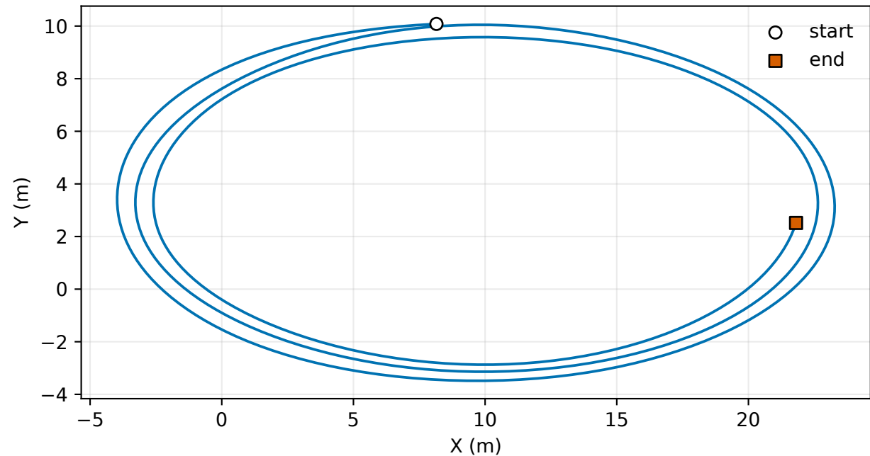
Q2 asynchronous KF/RTS fused trajectory at 10 Hz
