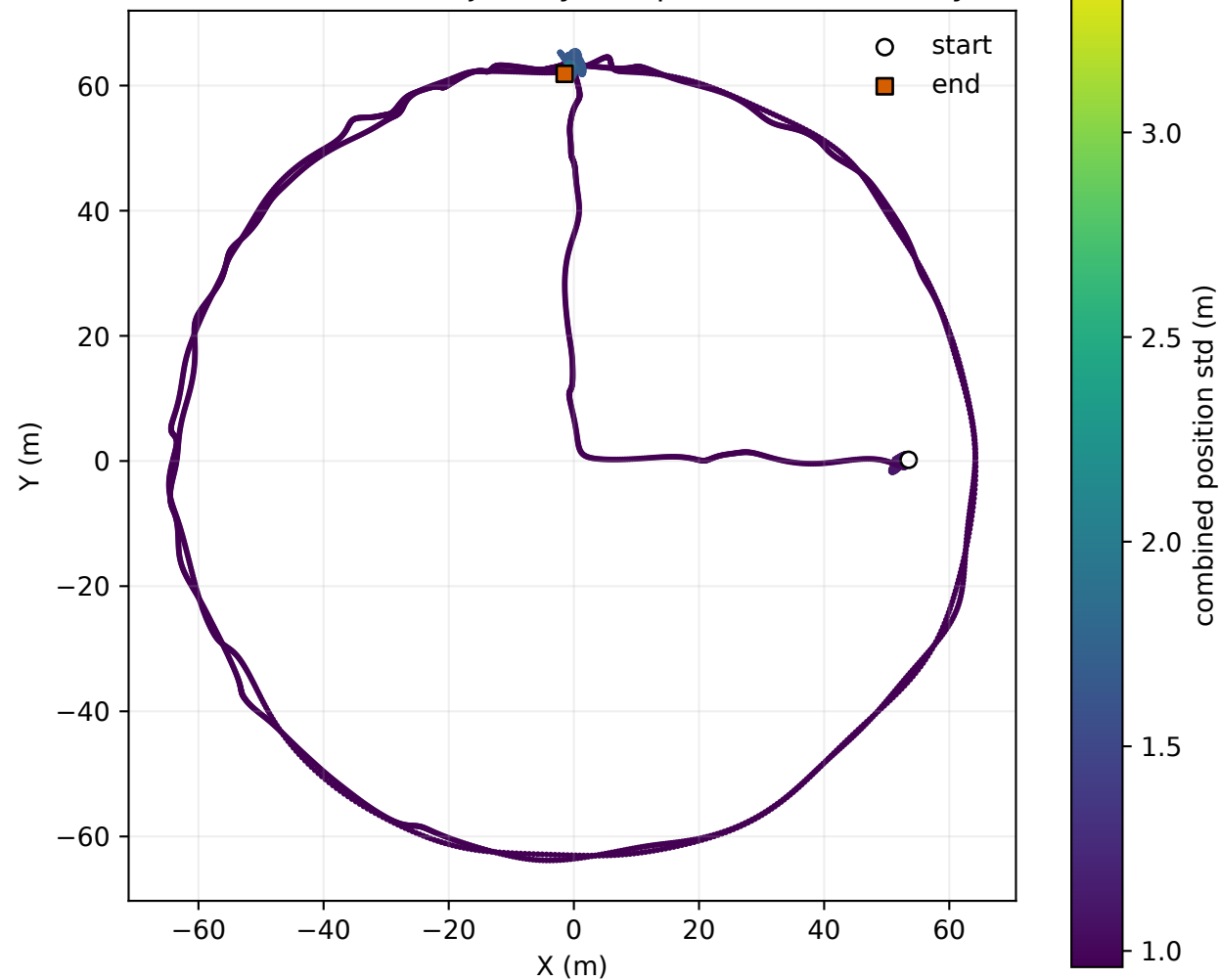
Q3 10 Hz fused trajectory and position uncertainty
