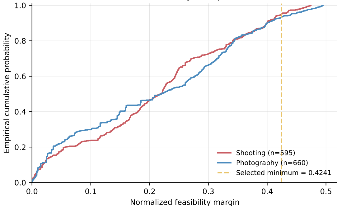
Q4 candidate-margin empirical CDF
