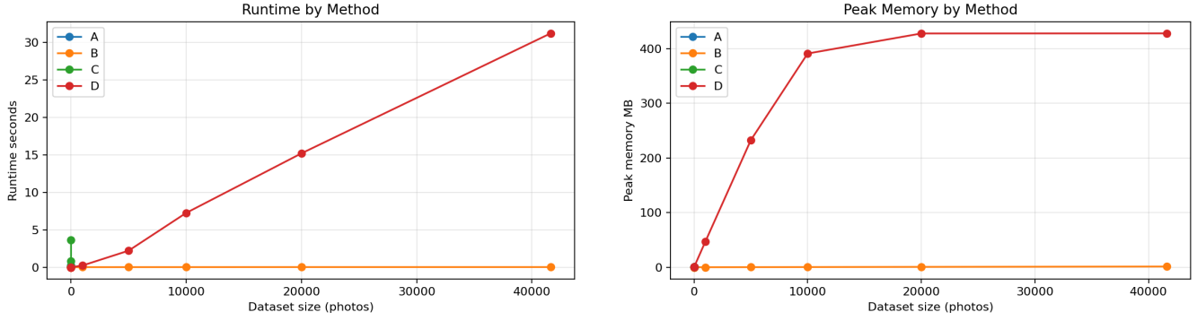
Figure 3: Runtime and peak measured memory by method and dataset size. Exact methods appear only on tiny samples; B is effectively instantaneous, while D pays more runtime and memory for embedding coverage.
