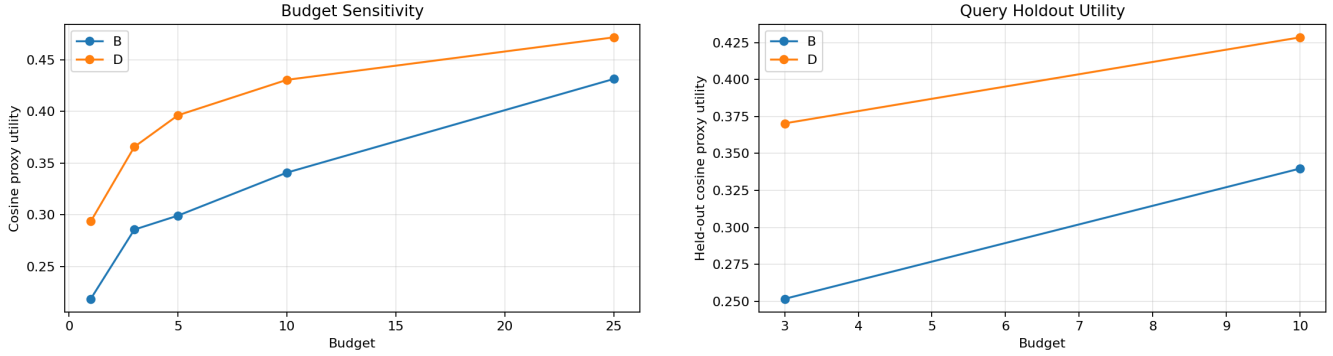
Figure 4: Budget sensitivity and held-out query utility. D gains more embedding-level utility as the retention budget grows and remains stronger than B on held-out queries.
