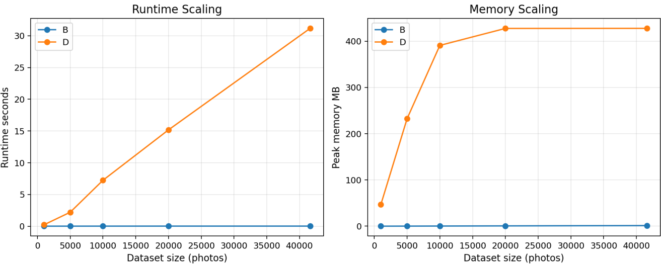
Figure 2: Runtime and memory scaling for Methods B and D. Method D is more expensive but remains feasible on the full dataset through chunked similarity coverage.
