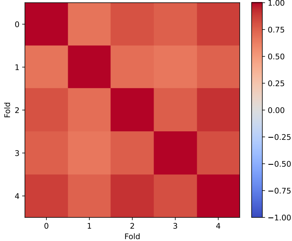
Channel-rank stability by fold
