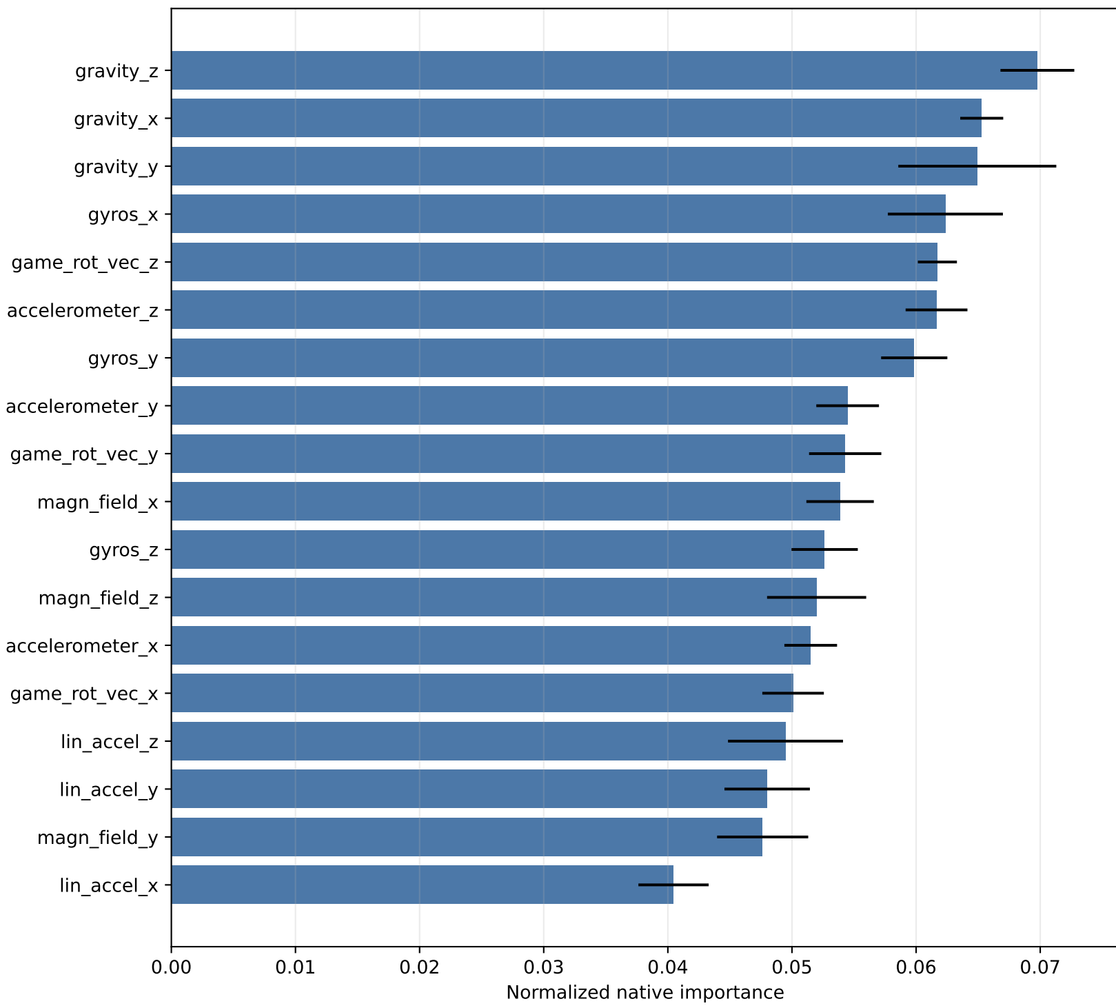
Ranked sensor-axis channel contribution
