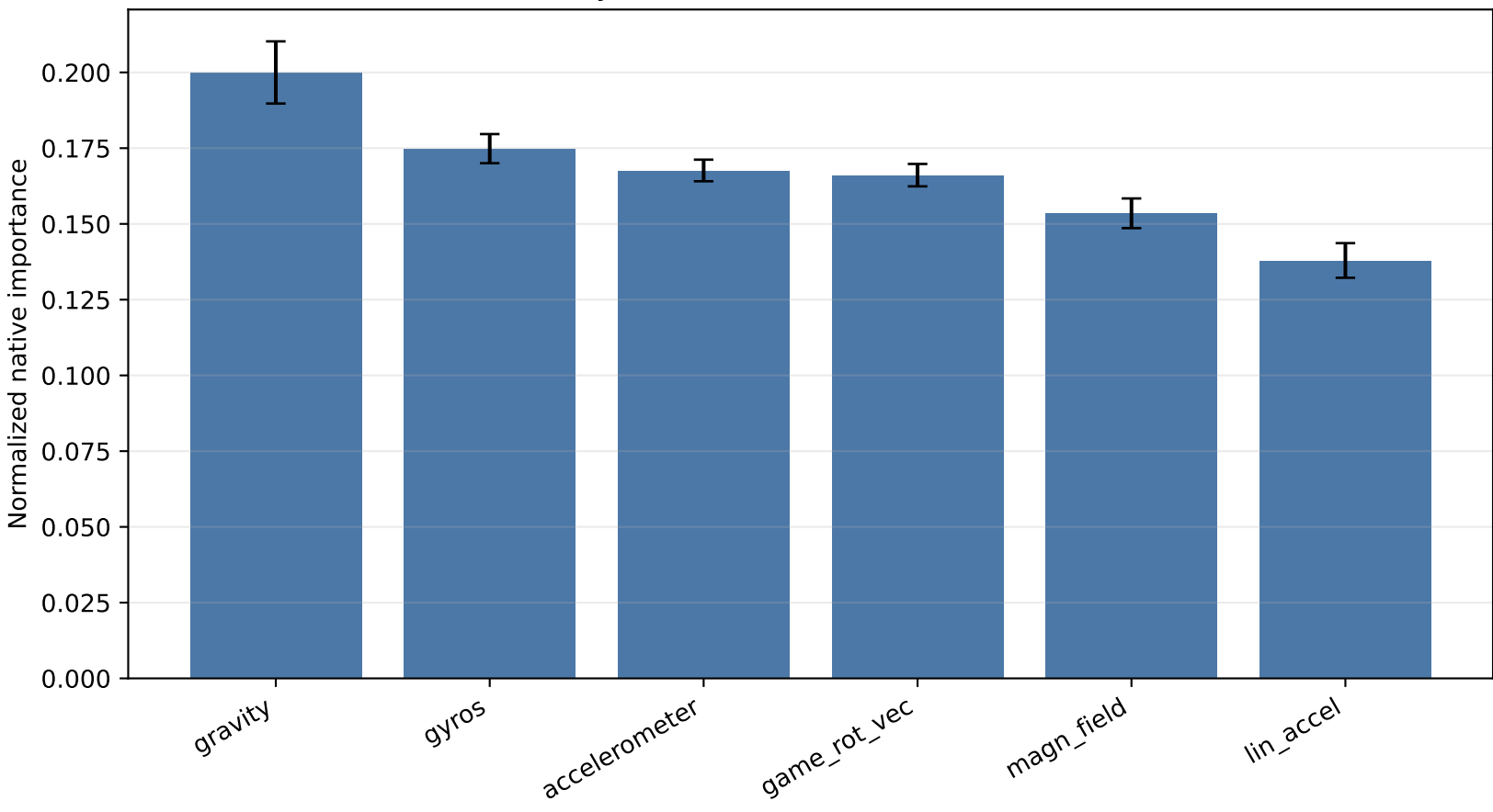
Sensor-family contribution to movement classification
