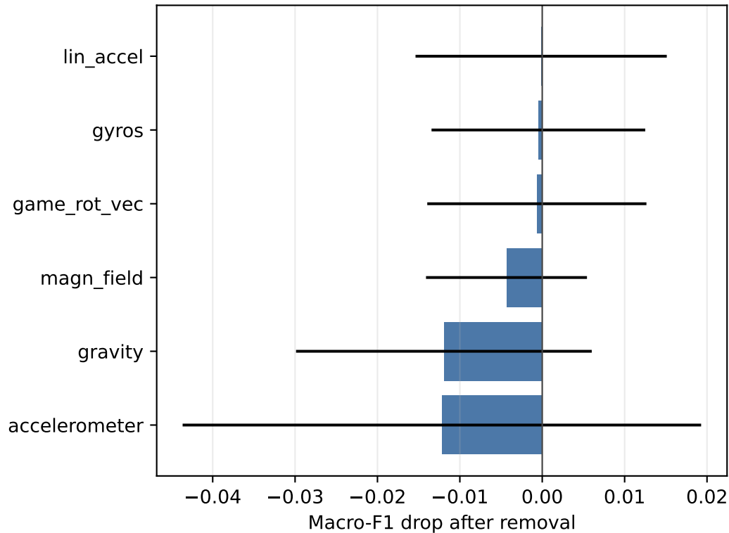
Sensor-family ablation
