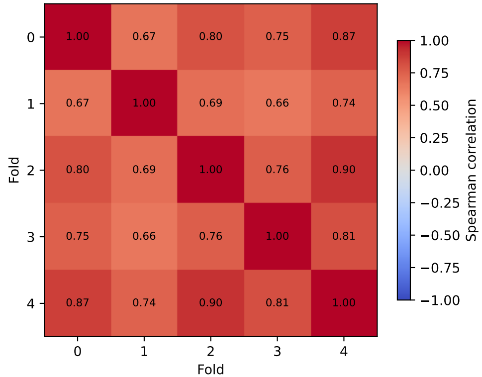
Channel-rank stability
