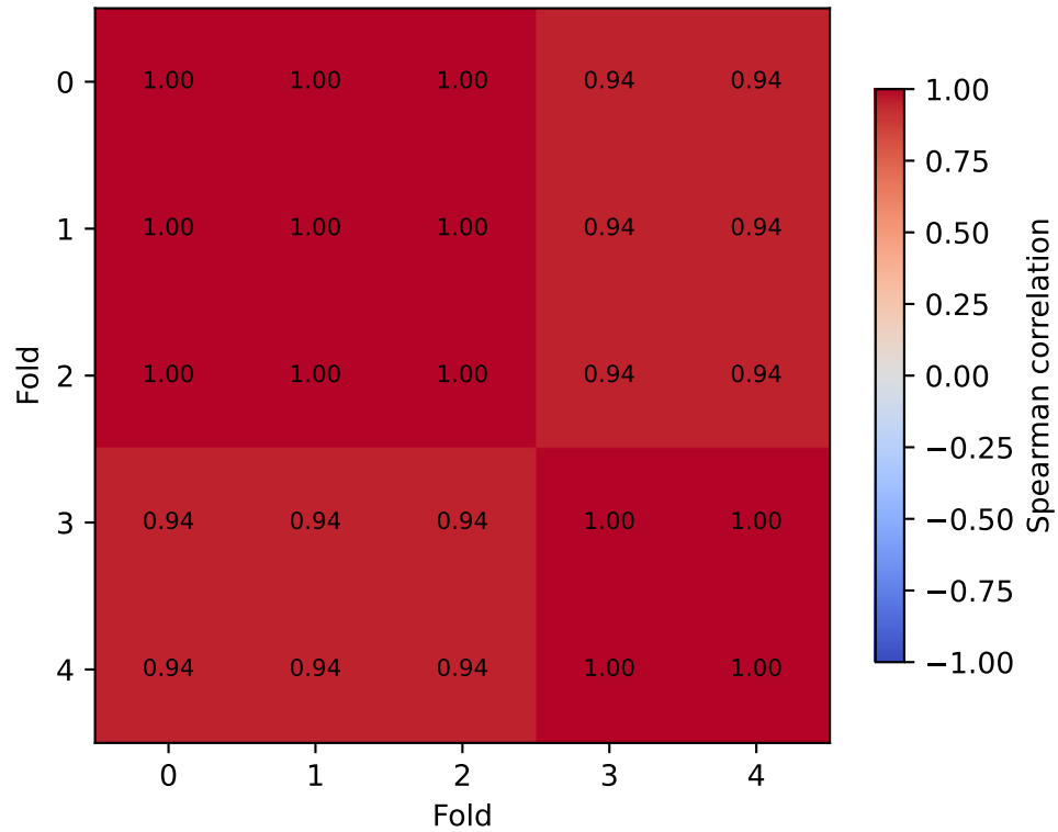
Dilation-rank stability
