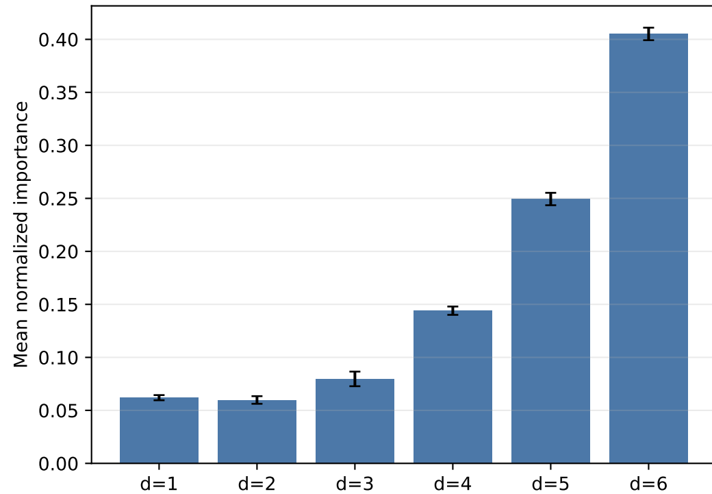
Dilation importance
