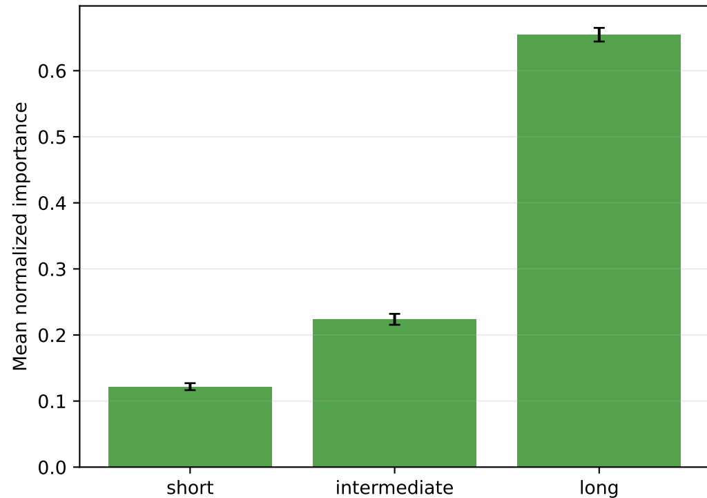
Temporal-scale bins
