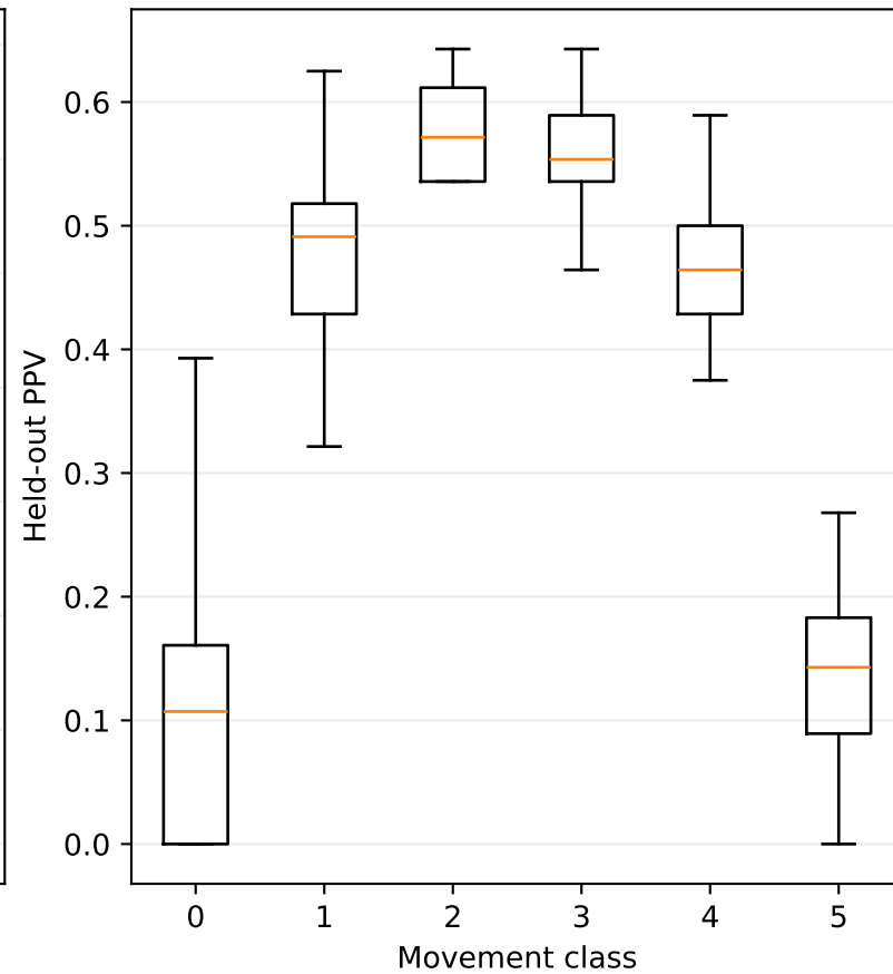
Feature 7931
