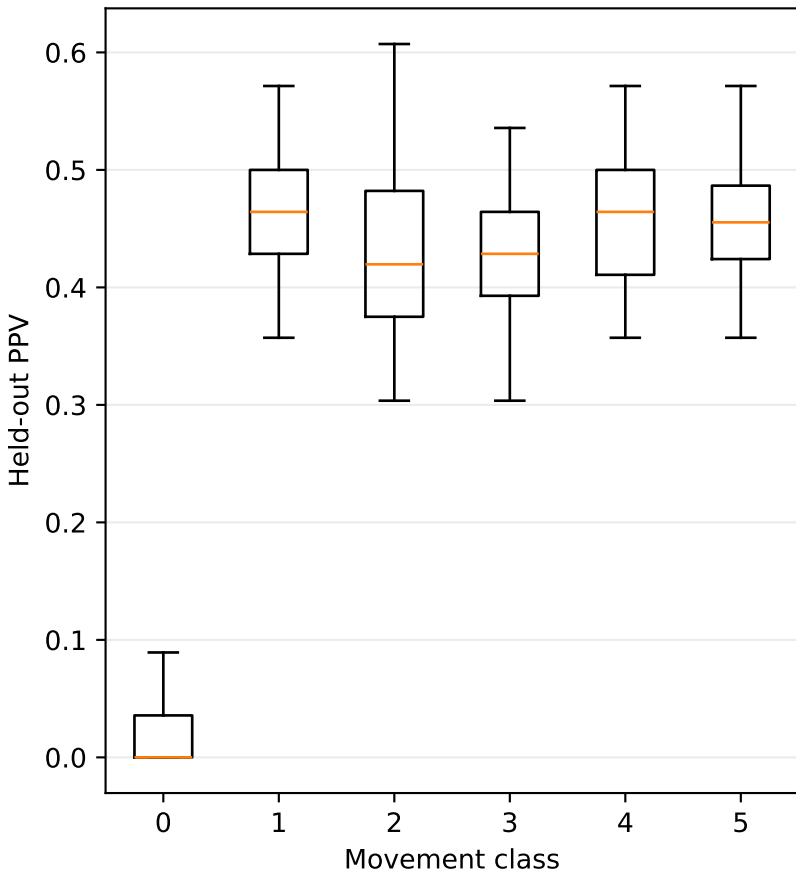
Feature 8164
