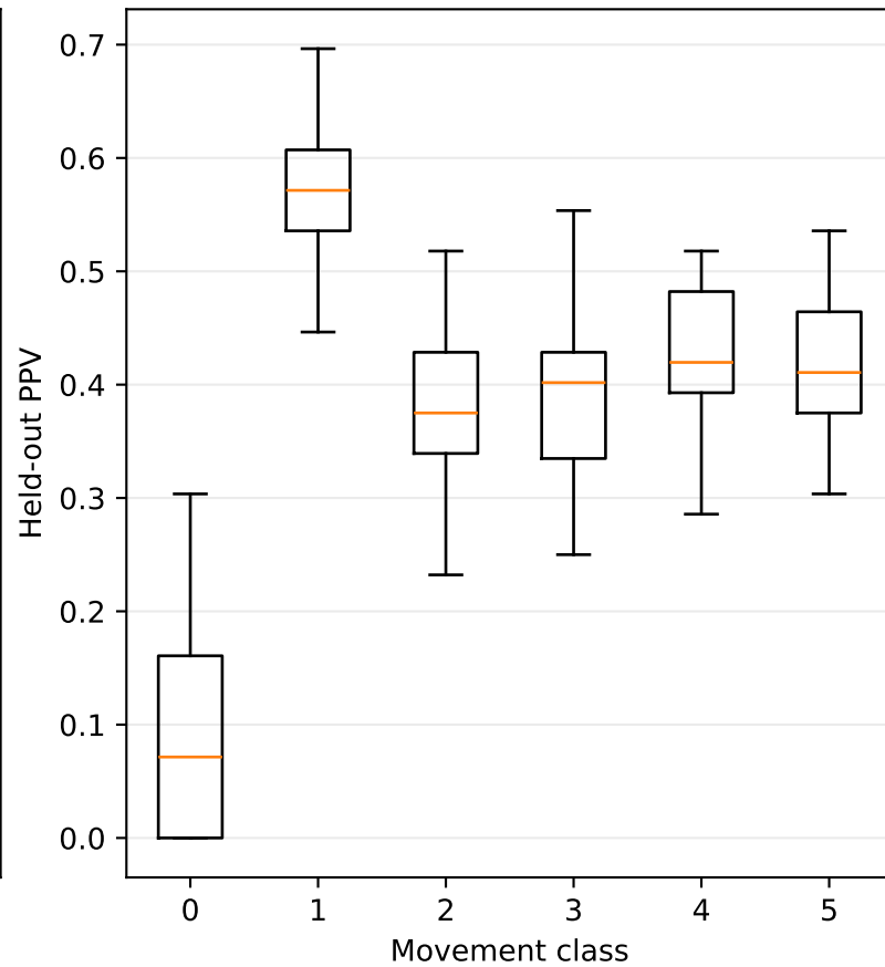
Feature 8429
