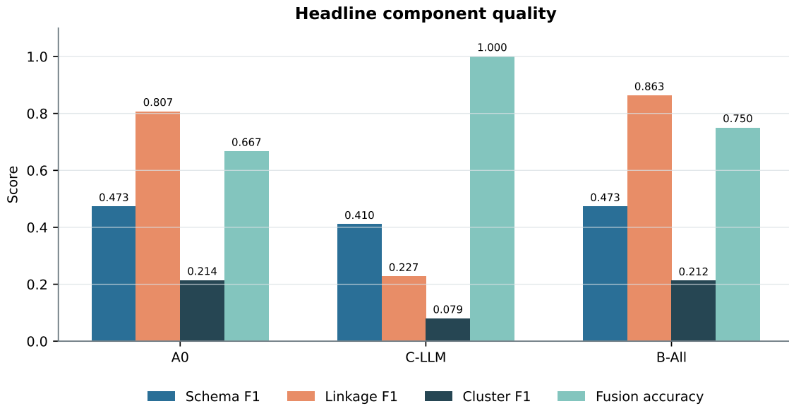
Figure 1: Headline component quality for the deterministic, LLM-primary, and hybrid pipelines. Exact values are retained in Table 3.
