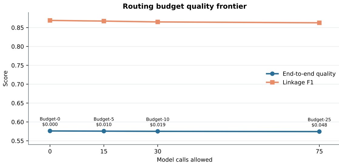
Figure 5: Routing-budget frontier. Labels show the configuration and estimated model cost at each call cap.
