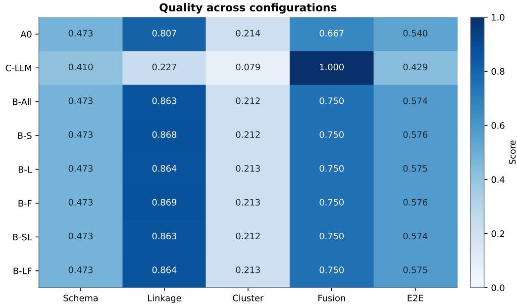
Figure 2: Quality matrix for the baseline, LLM-primary, hybrid, and stage-ablation configurations. Exact values remain available in the release metrics CSV.
