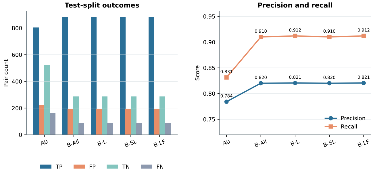
Figure 3: Linkage test outcomes and precision-recall comparison for the baseline and linkage-assisted configurations.
