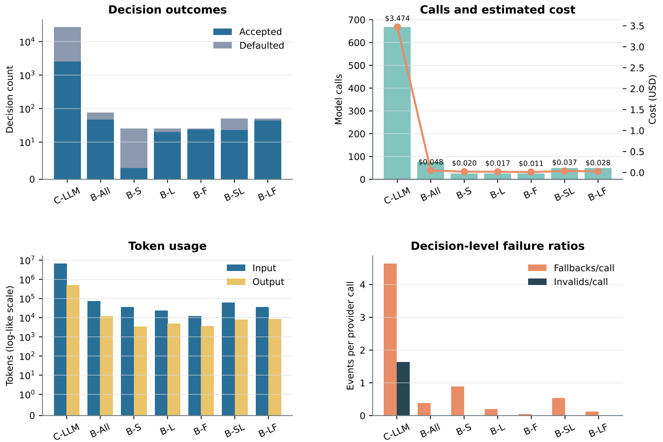
Figure 4: Operational dashboard for LLM-primary, hybrid, and stage-ablation runs. Logarithmic axes preserve readability across the large difference between C-LLM and selectively routed configurations.
