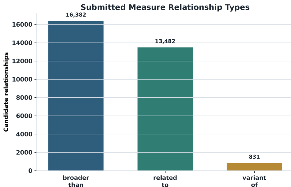
Figure 6. Submitted Step 8 relation type distribution.
