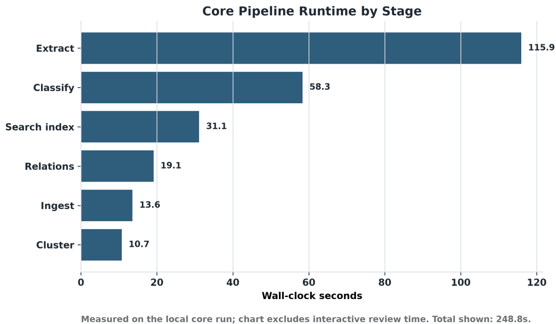
Figure 7. Core pipeline wall-clock runtime by stage.
