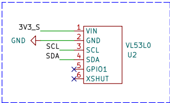
TOF sensor
