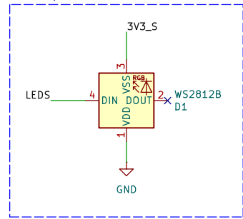
Leds strips
