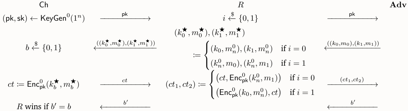
Figure 2: Experiment \text{PKE}_{\Pi^0}^{\text{IND-CPA}}
