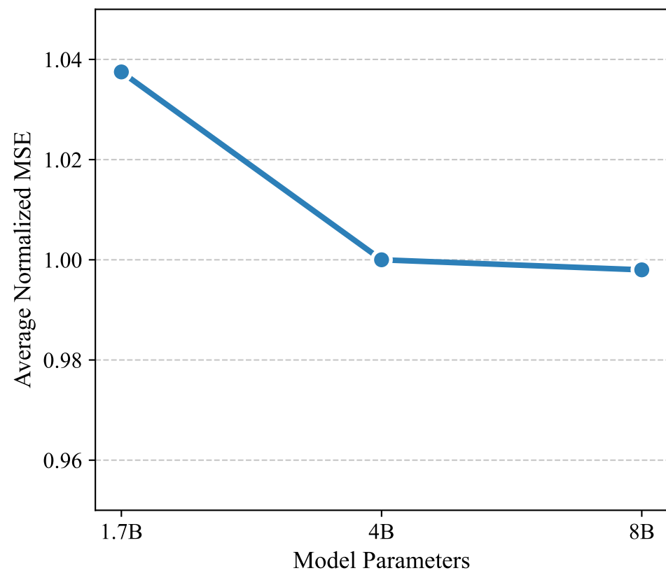
(a) Scaling Law in Qwen3 Family
