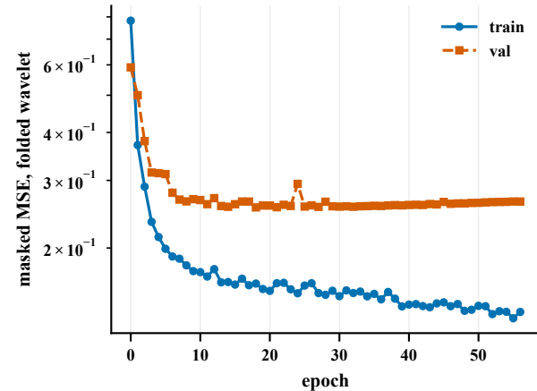
Spec reconstruction
