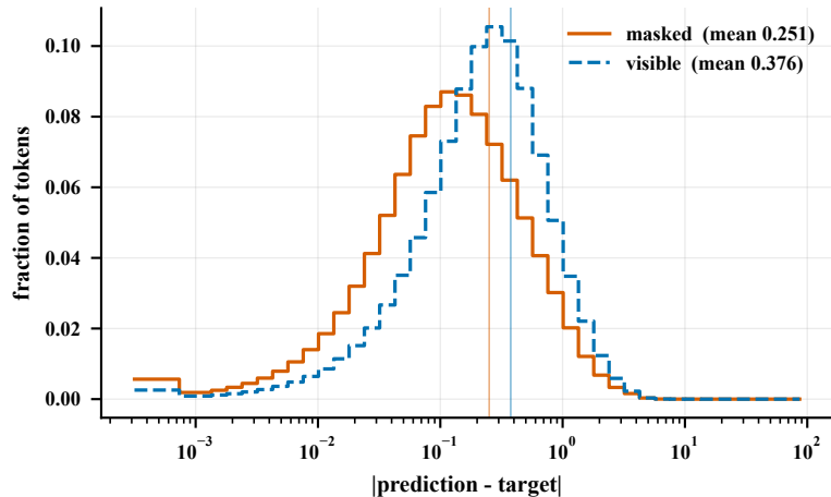
Folded-wavelet patches
