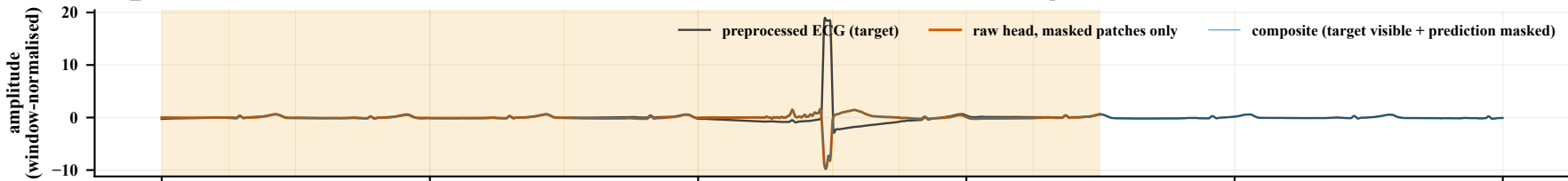
L12_500 code15 channel I window 0 r -0.931 NMSE 2.111 MAE 0.582 RMSE 2.604 masked 14/20 patches
