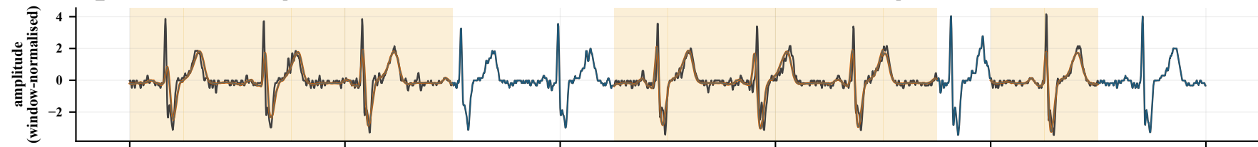
L1_250 icentia11k channel patch1 window 0 r 0.830 NMSE 0.314 MAE 0.284 RMSE 0.532 masked 14/20 patches
