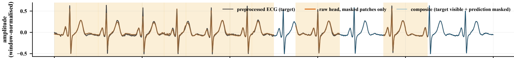
L12_500 code15 channel I window 6413 r 0.985 NMSE 0.033 MAE 0.017 RMSE 0.025 masked 14/20 patches
