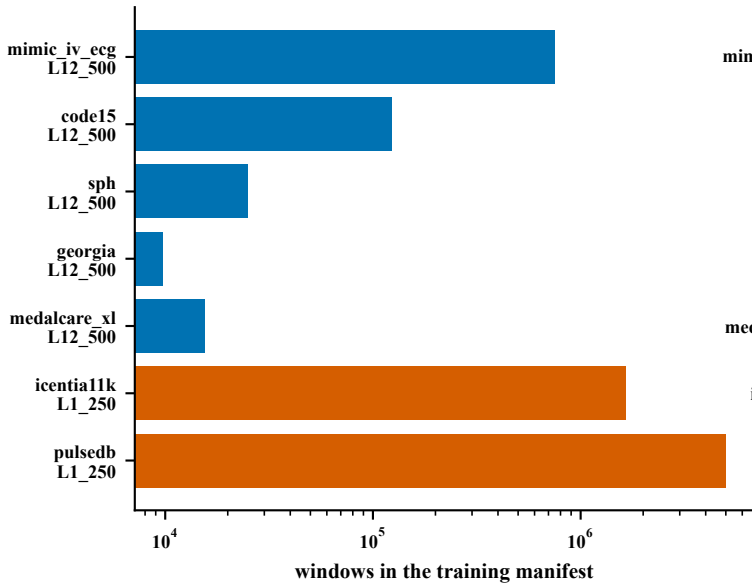
corpus size by dataset
