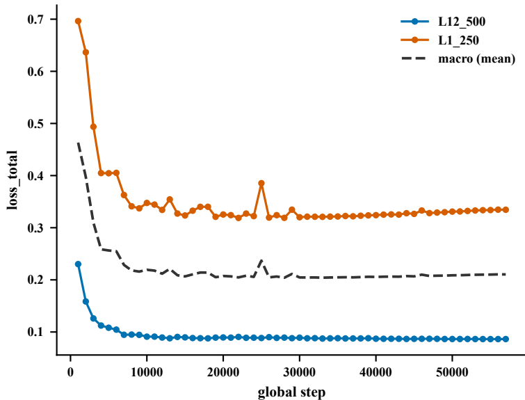
validation loss_total, by route
