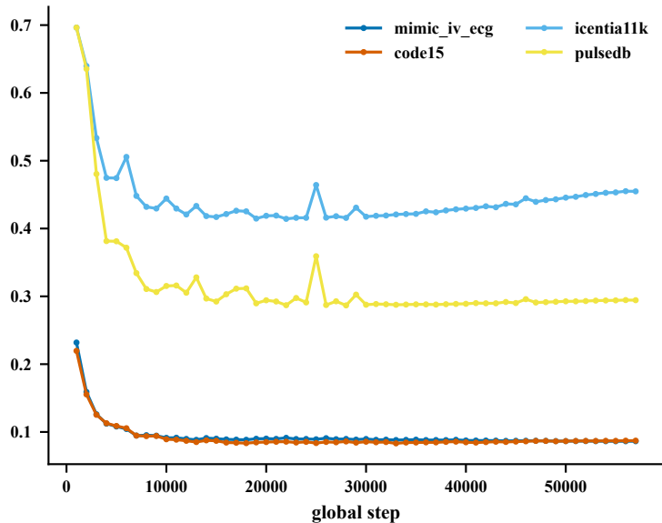
validation loss_total, by dataset (supplementary)
