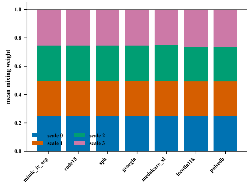
ScaleFold alpha by dataset (a single full bar = collapse onto one scale)
