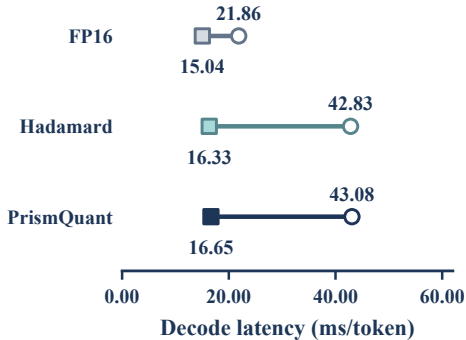
a Llama-3.2-3B decode Private current-stream backend
