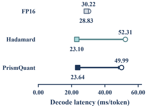
b Llama-3.1-8B decode Private current-stream backend
