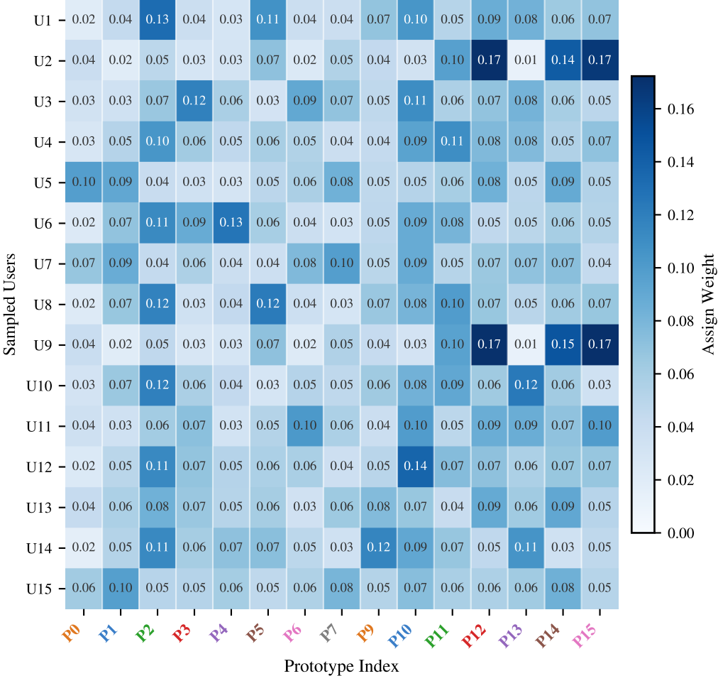
User-Prototype Assignment Pattern (1 user per prototype, shuffled order)
