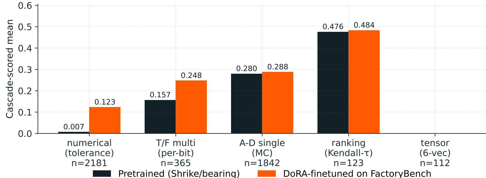
FactoryBench performance by answer format — bearing_mixed_r32, L1-L3
