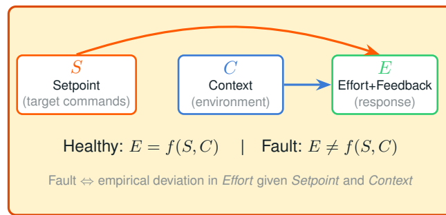
Figure 6: Physical causal schema. Setpoint commands S and contextual variables C jointly determine the measured Effort + Feedback response E under healthy operation. Faults manifest as residuals E - f(S, C) from this nominal mapping.
