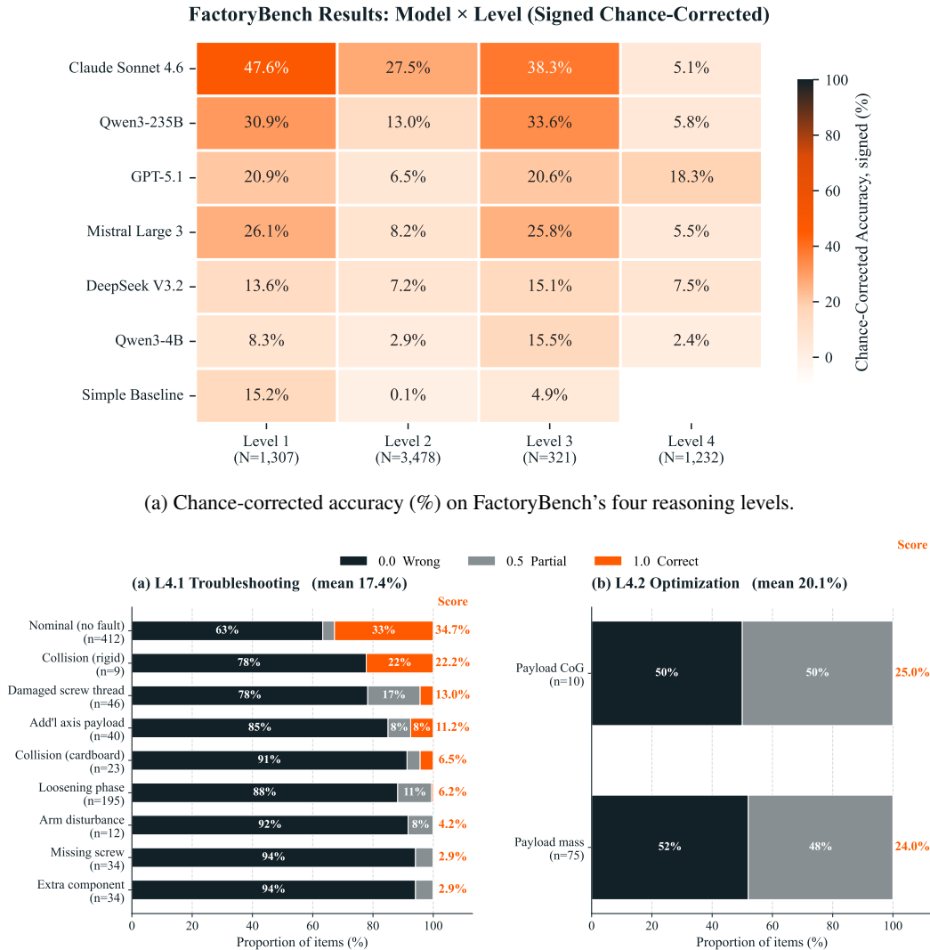
(b) GPT-5.1 L4 score distribution by ground-truth root cause (left, troubleshooting) and misconfigured parameter (right, optimization). Each bar shows the proportion of items scored 0/0.5/1; the right-edge value is the per-category mean accuracy.
