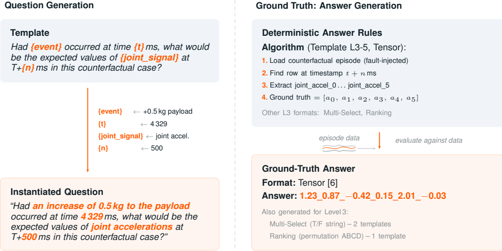
Figure 2: Question-and-answer generation pipeline, illustrated with Level 3 Template 5 (counterfactual tensor prediction) out of 20 templates total (see Table 7 for the full inventory and Appendix E for worked examples). Left: A parameterised template defines the question skeleton with typed placeholder slots ( orange ); slot binding maps each placeholder to a concrete value sampled from the episode context, yielding an instantiated question . Right: Ground-truth answers are computed deterministically: template-specific rules extract the answer from paired episode data, producing the ground-truth answer without manual annotation.
