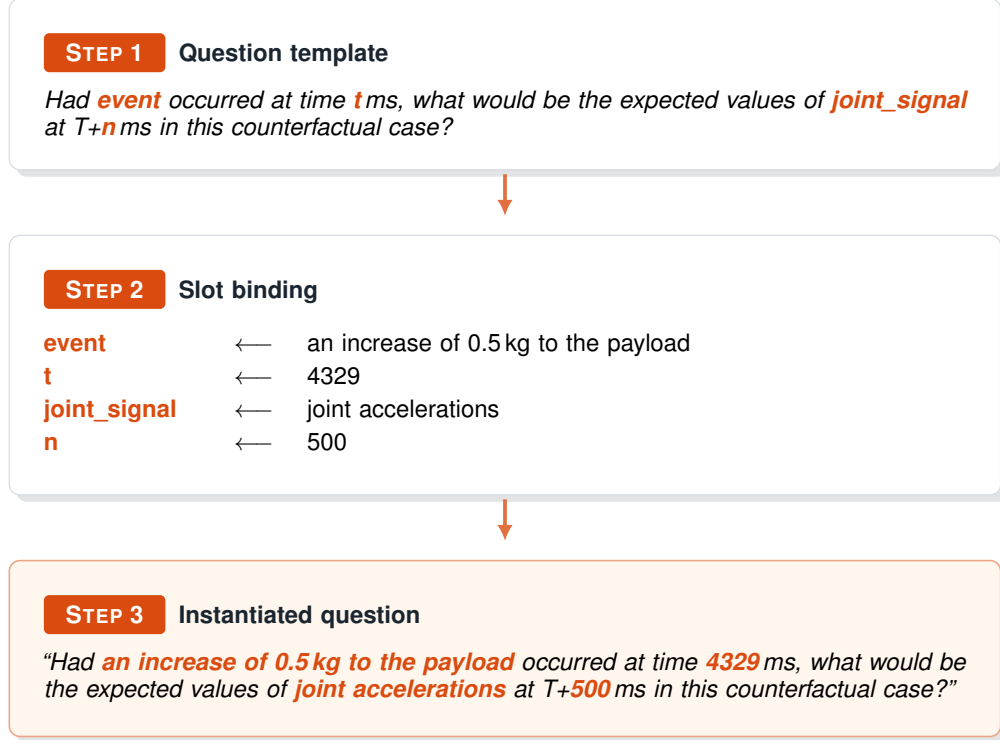
Figure 2: The question-generation pipeline. A parameterised template (Step 1) defines the question skeleton with typed placeholder slots. Slot binding (Step 2) maps each placeholder to a concrete value sampled from the scenario context. The resulting instantiated question (Step 3) is ready for inclusion in the FactoryBench Q&A dataset.
