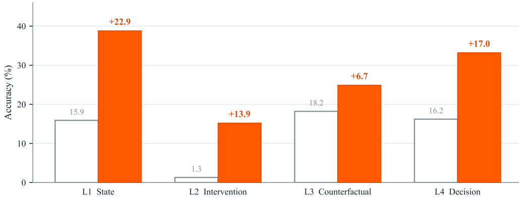
Figure 9: A three-step loop, and the lift it produces. (a) The agent as a state machine. The driver cycles through three states, reason, call a tool, read the result, and re-enters the cycle at most six times before leaving it to answer. Tools are reachable only from the calling state. Nothing is tuned on FactoryBench. (b) Accuracy per level for GPT-5.1 zero-shot and for the same model given those tools, on an 800-item stratified subset; L1 and L2 more than double. L1–L3 are signed chance-corrected; L4 uses the uncorrected free-form judge rubric and is not comparable across the L4 boundary.
