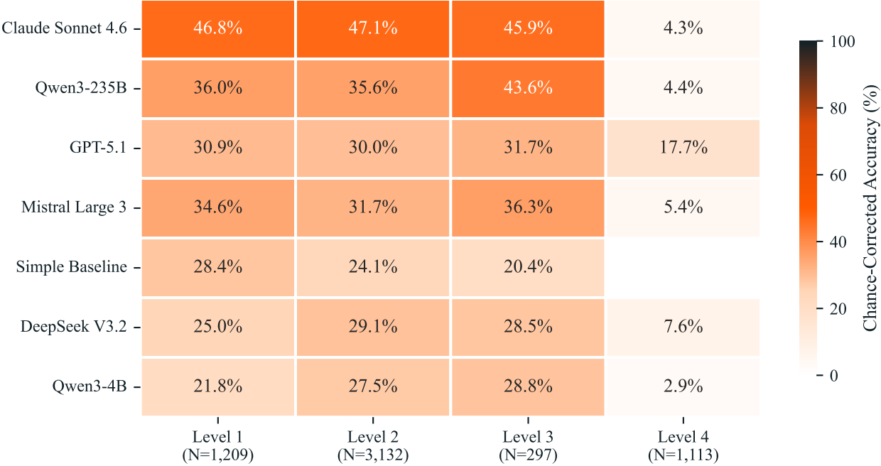
FactoryBench Results: Model × Level (Chance-Corrected)
