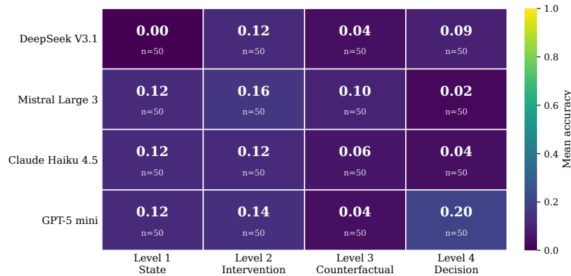
Figure 3: Measured accuracy of four frontier models evaluated via Microsoft Foundry across FactoryBench’s four reasoning levels. Each cell reports the mean accuracy over n evaluated Q&A pairs. Levels 1–3 and Level 4 ranking templates use deterministic scoring; Level 4 free-form templates (troubleshooting and optimization) are scored against the reference root cause and remediation protocol under a \{0, 0.5, 1\} rubric.
