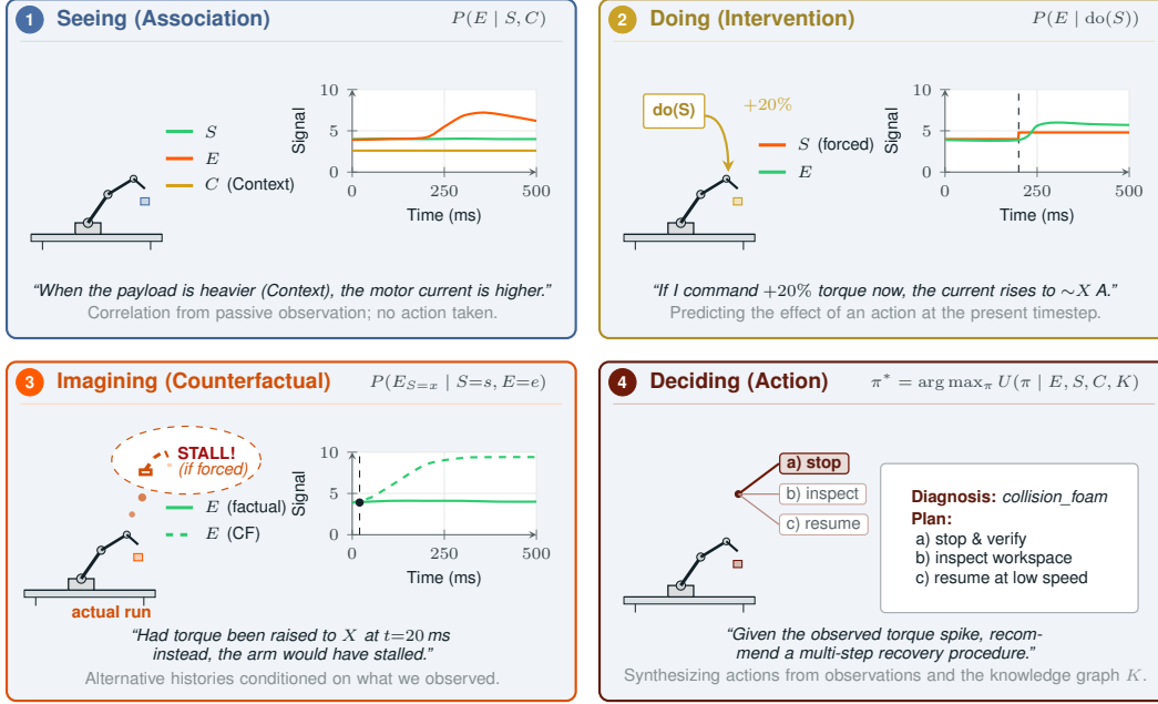
Figure 1: Pearl’s three rungs of causal reasoning (L1–L3), instantiated on robotic time-series, plus the FactoryBench L4 decision-making layer. Signals follow the SCE schema (Section 3.3): S is the setpoint (the controller’s commanded target), E is the effort (the machine’s measured response, e.g., motor current or torque), and C is the context (physical and configured operating conditions, e.g., payload mass). L1 (Seeing) captures correlations from passive observation; L2 (Doing) predicts the effect of an intervention; L3 (Imagining) reasons over alternative histories conditioned on what was observed; L4 (Deciding) synthesizes a recovery procedure by combining the observed signals with manufacturer manuals and the FactoryBench knowledge graph K .
