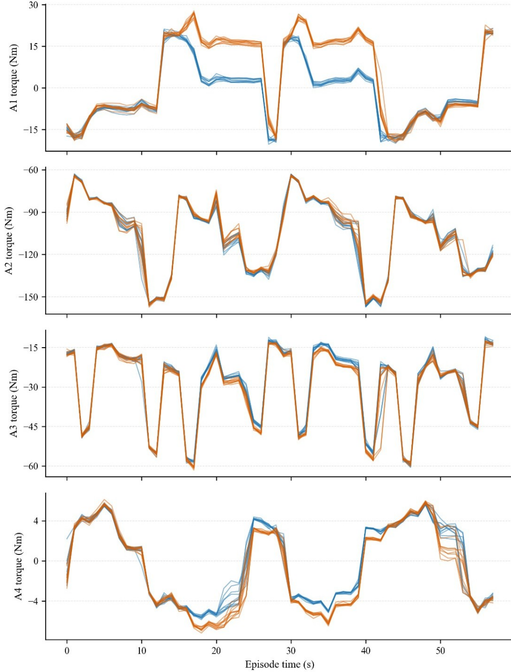
Figure 8: Sensor data distribution across multiple healthy KUKA episodes (blue) versus multiple faulty episodes with an arm-disturbance fault (orange) in FactoryWave. The visible shift between the two groups confirms that templates with small noise-substitution \Delta are still solvable from the released signal; the magnitude of the shift varies across joints because the disturbance angle loads them unequally.
