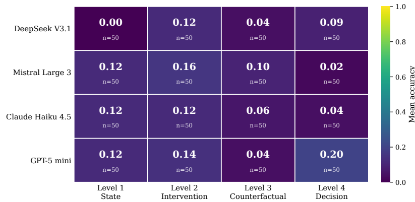
Figure 4: Measured accuracy of four frontier models evaluated via Microsoft Foundry across FactoryBench’s four reasoning levels. Each cell reports the mean accuracy over n evaluated Q&A pairs. Levels 1–3 and Level 4 ranking templates use deterministic scoring; Level 4 free-form templates (troubleshooting and optimization) are scored against the reference root cause and remediation protocol under a \{0, 0.5, 1\} rubric.
